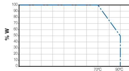
CER14 Through-hole
