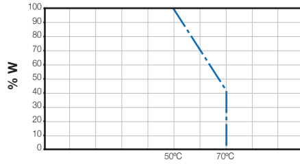
CA9 Through-hole and SMD
