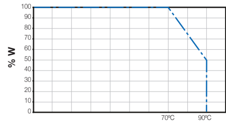
MCE9 Through-hole
