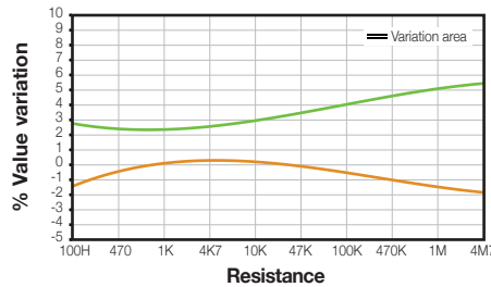
CA9 Through-hole and SMD
