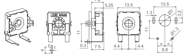
VSMD...CY
